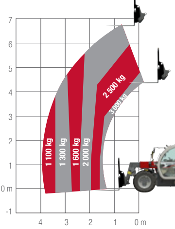
MF TH.7030
