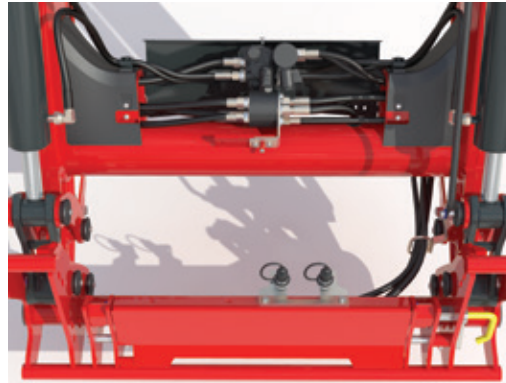
Cross-tube houses hydraulic components and provides strength without impacting the visibility
