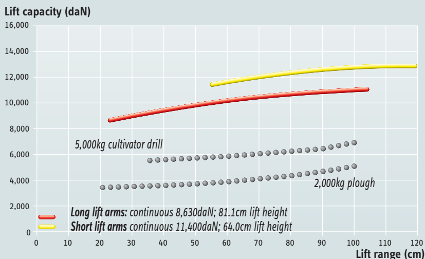
Massey Ferguson 8690: The red curve shows the recorded lift capacity (90% of maximum lift) as continuous lift power on the link ends. The yellow curve displays lift capacity with lift arms shortened – more than 2,770daN extra lift capacity, 17cm smaller lift range. Our MF test candidate boasted excellent lift forces.
